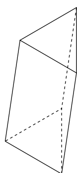
Triangular prism
